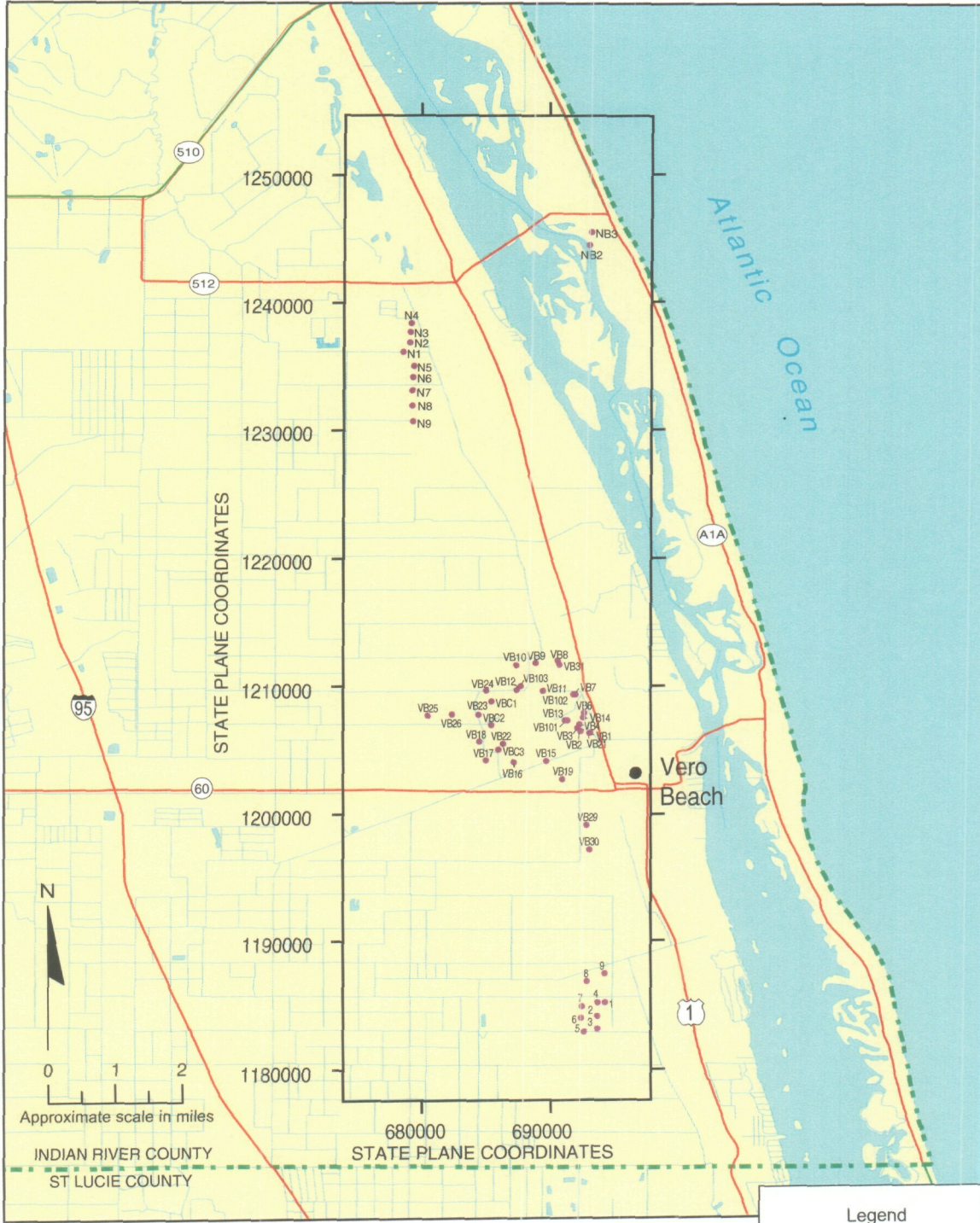
Figure 1. Model area for Vero Beach and Indian River County wellfields
